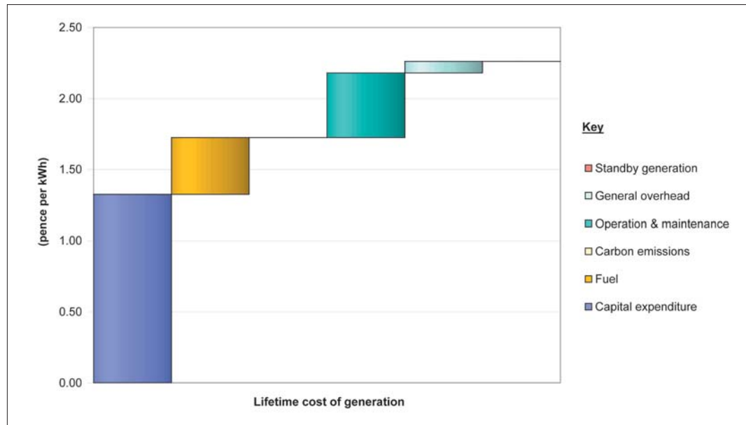
Figure A.9 - Current cost of generating electricity from nuclear fission plant
