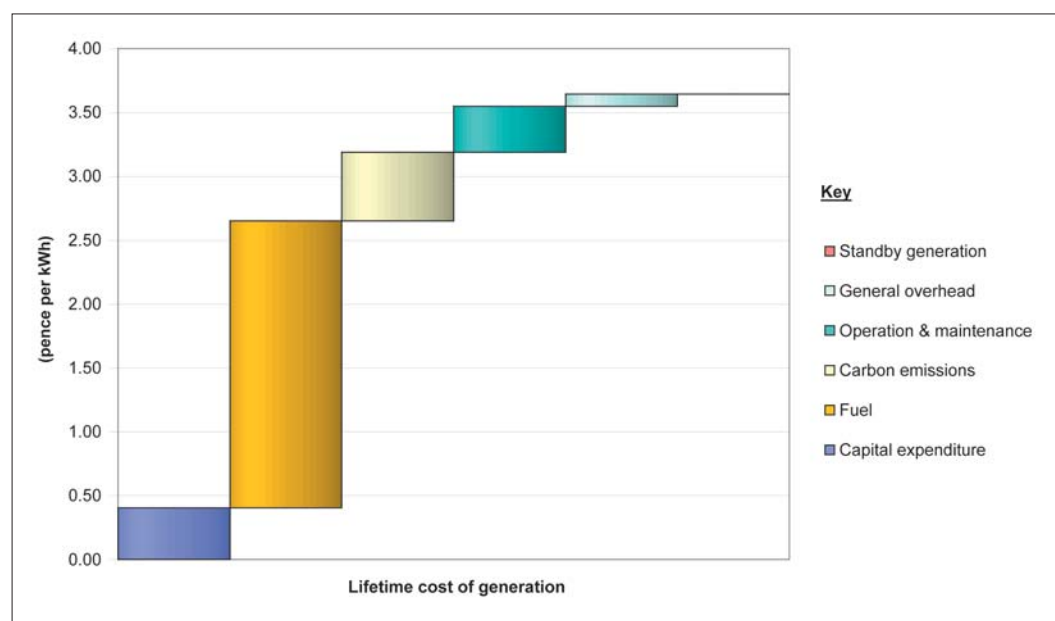
Figure A.6 – Current cost of generating electricity from gas-fired OCGT plant
