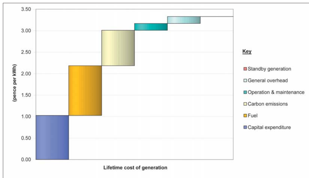
Figure A.1 – Current cost of generating electricity from coal-fired PF plant.
