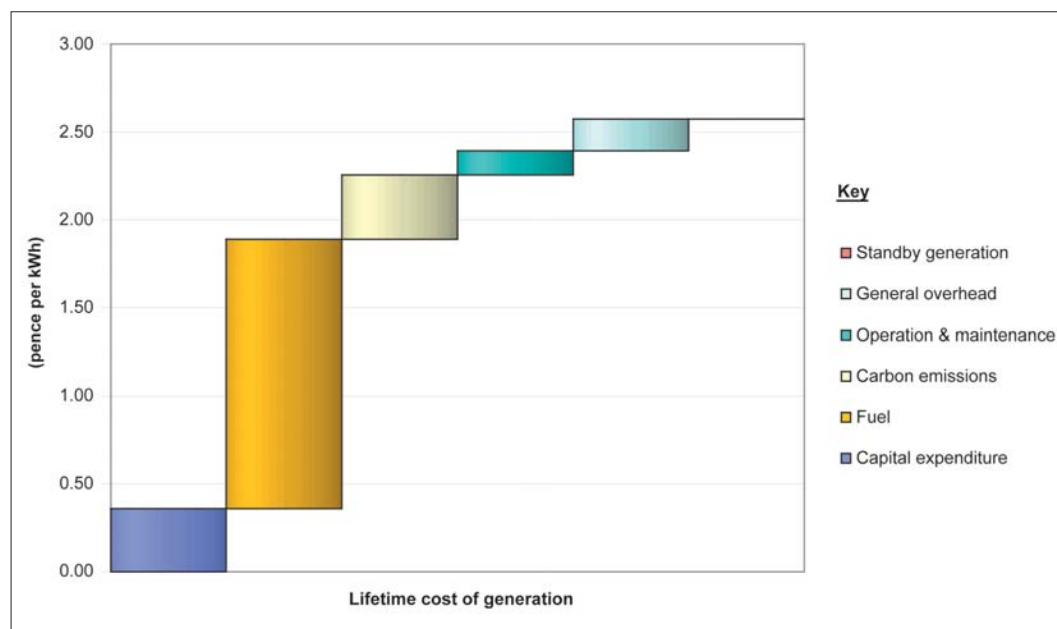
Figure A.8 – Current cost of generating electricity from gas-fired CCGT plant
