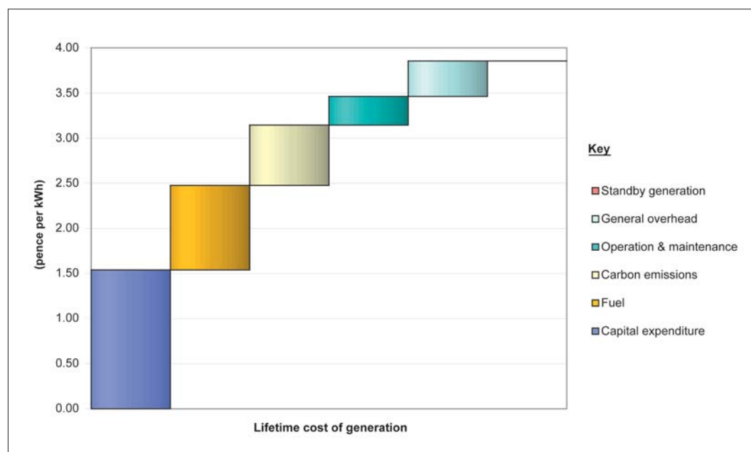
Figure A.4 – Current cost of generating electricity from coal-fired IGCC plant
