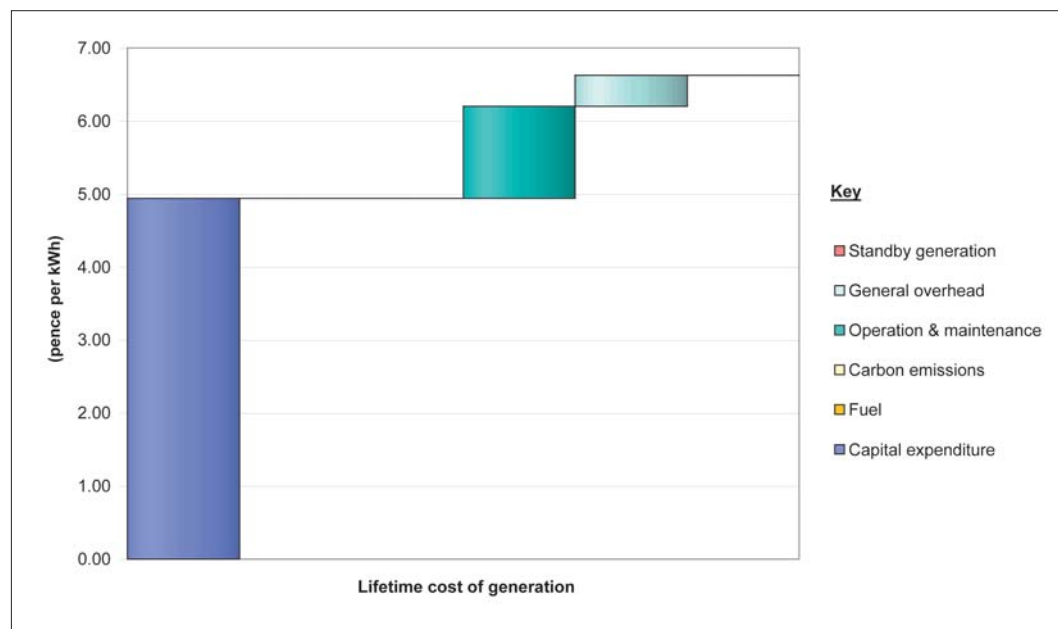
Figure A.12 Current cost of generating electricity from wave and marine technologies
