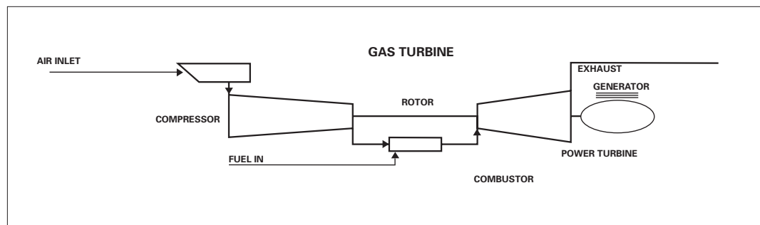
Figure A.5 – Typical OCGT configuration
