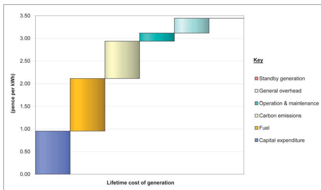
Figure A.2 – Current cost of generating electricity from coal-fired CFB plant
