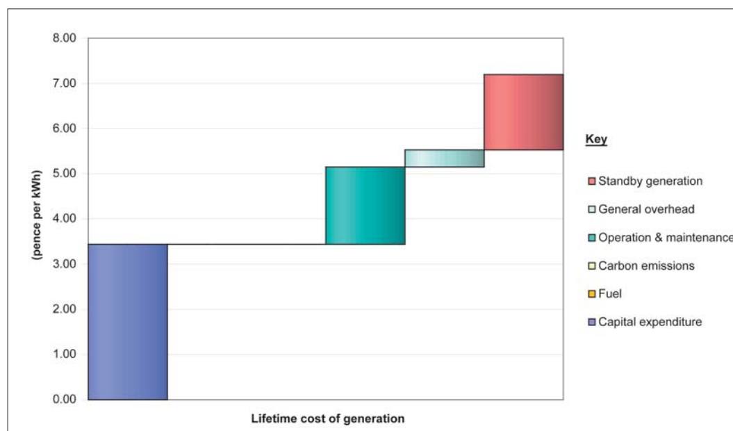
Figure A.11 – Current cost of generating electricity from offshore wind farms
