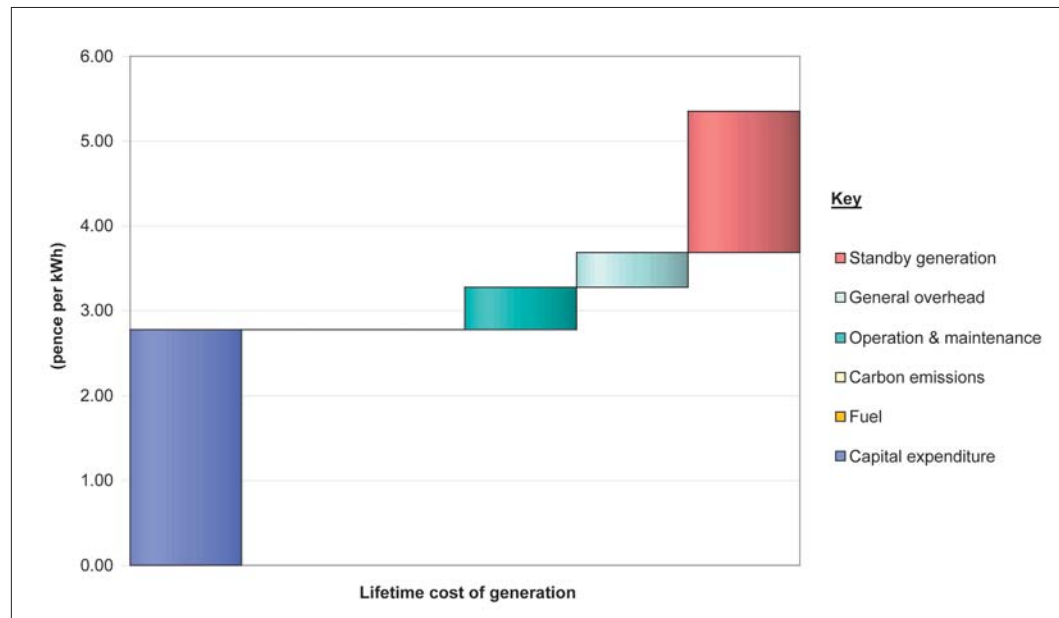
Figure A.10 – Current cost of generating electricity from an onshore wind farm
