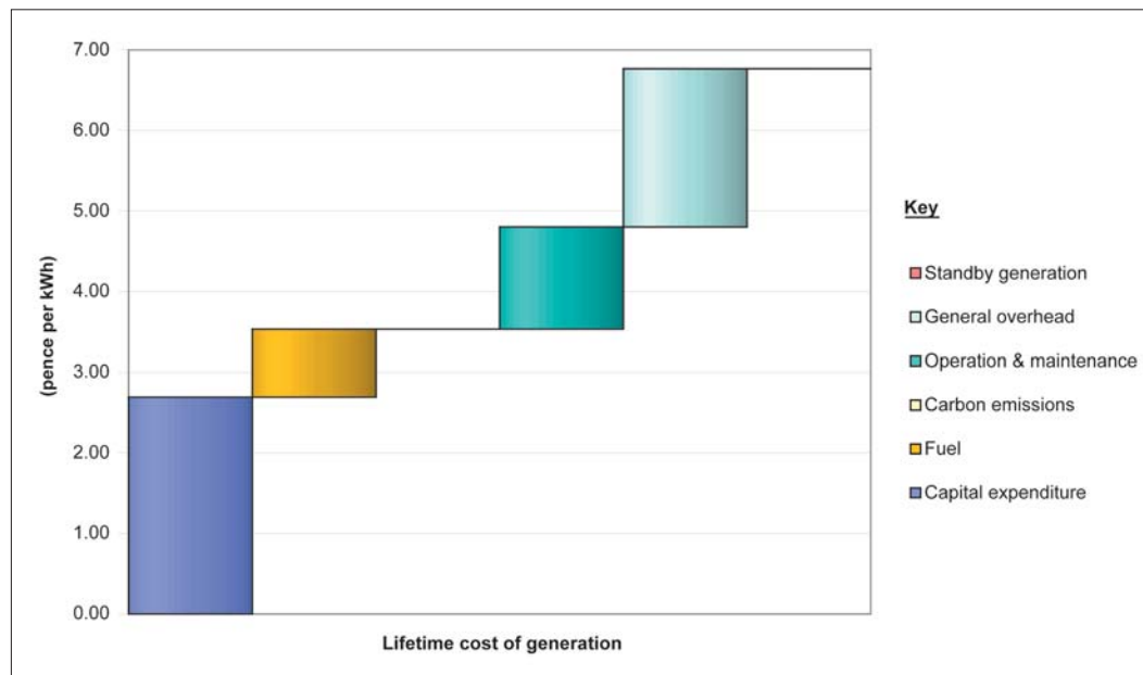
Figure A.3 – Current cost of generating electricity from biomass-fired BFB plant
