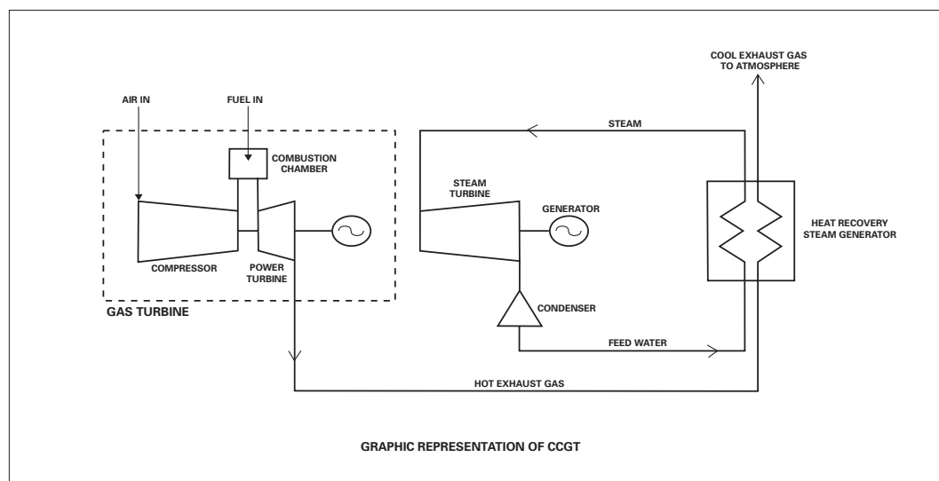
Figure A.7 – Typical CCGT configuration
