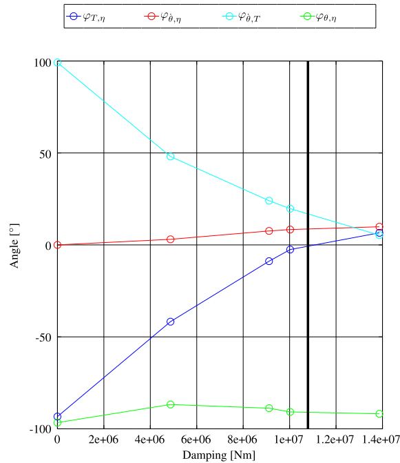
Fig. 10. Phase angles of kinetic properties over applied external damping T_{PTO} , with \varphi_{\phi_1,\phi_2} = \varphi_{\phi_1} - \varphi_{\phi_2} . The vertical black line indicates optimum damping ( H = 3 m).
