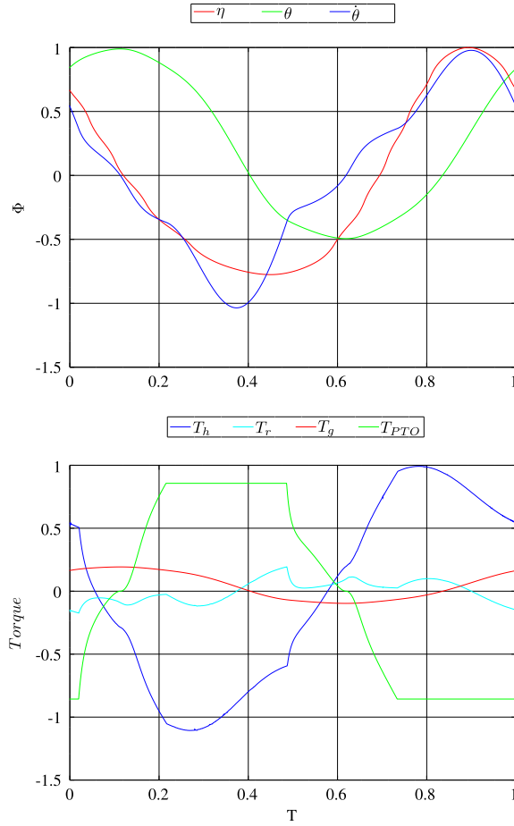
Fig. 4. Normalised surface elevation, kinematic quantities of the flap (top) and torque components (bottom) over one wave cycle for optimum damping as obtained from CFD simulations ( H = 2.1 m).
