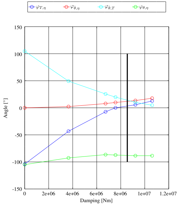
Fig. 9. Phase angles of kinetic properties over applied external damping T_{pto} , with \varphi_{\phi_1,\phi_2} = \varphi_{\phi_1} - \varphi_{\phi_2} . The vertical black line indicates optimum damping ( H = 2.1 m).
