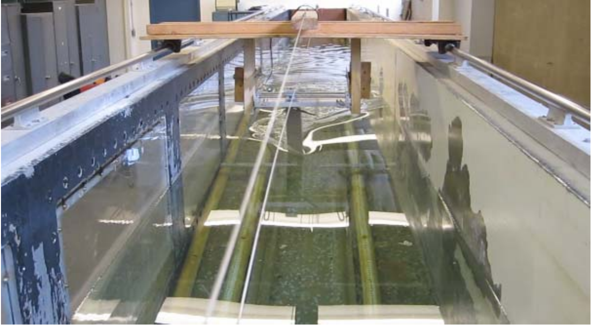
Figure 26. Towing Tank Run 1 Frame 364.
