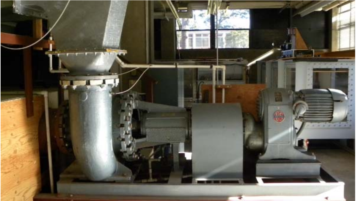
Figure 5. Water Tunnel One pump.
