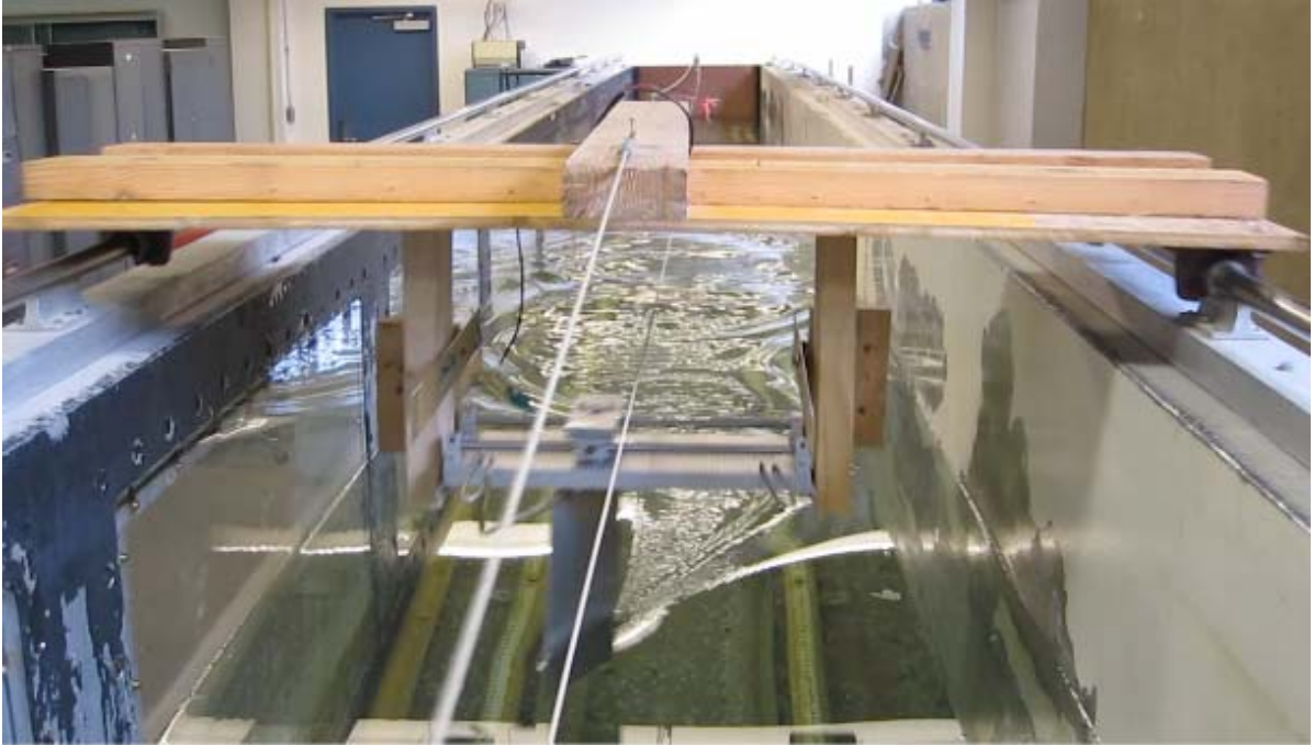
Figure 30. Towing Tank Run 1 Frame 392.
