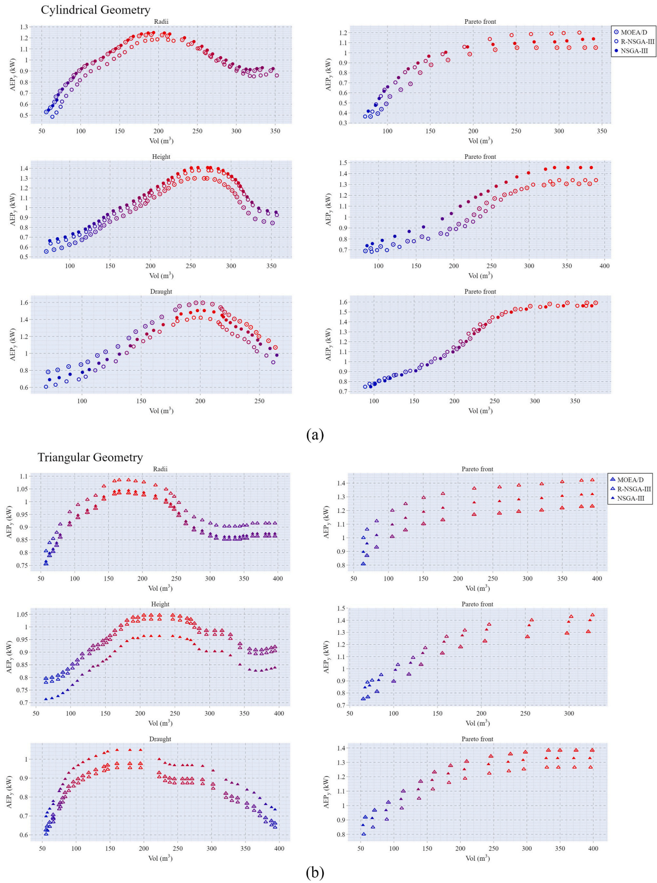
Fig. 14. AEP_y (left) and Pareto front (right) against the volume of (a) cylindrical, (b) triangular, (c) quadrilateral, and (d) octagonal geometries.
