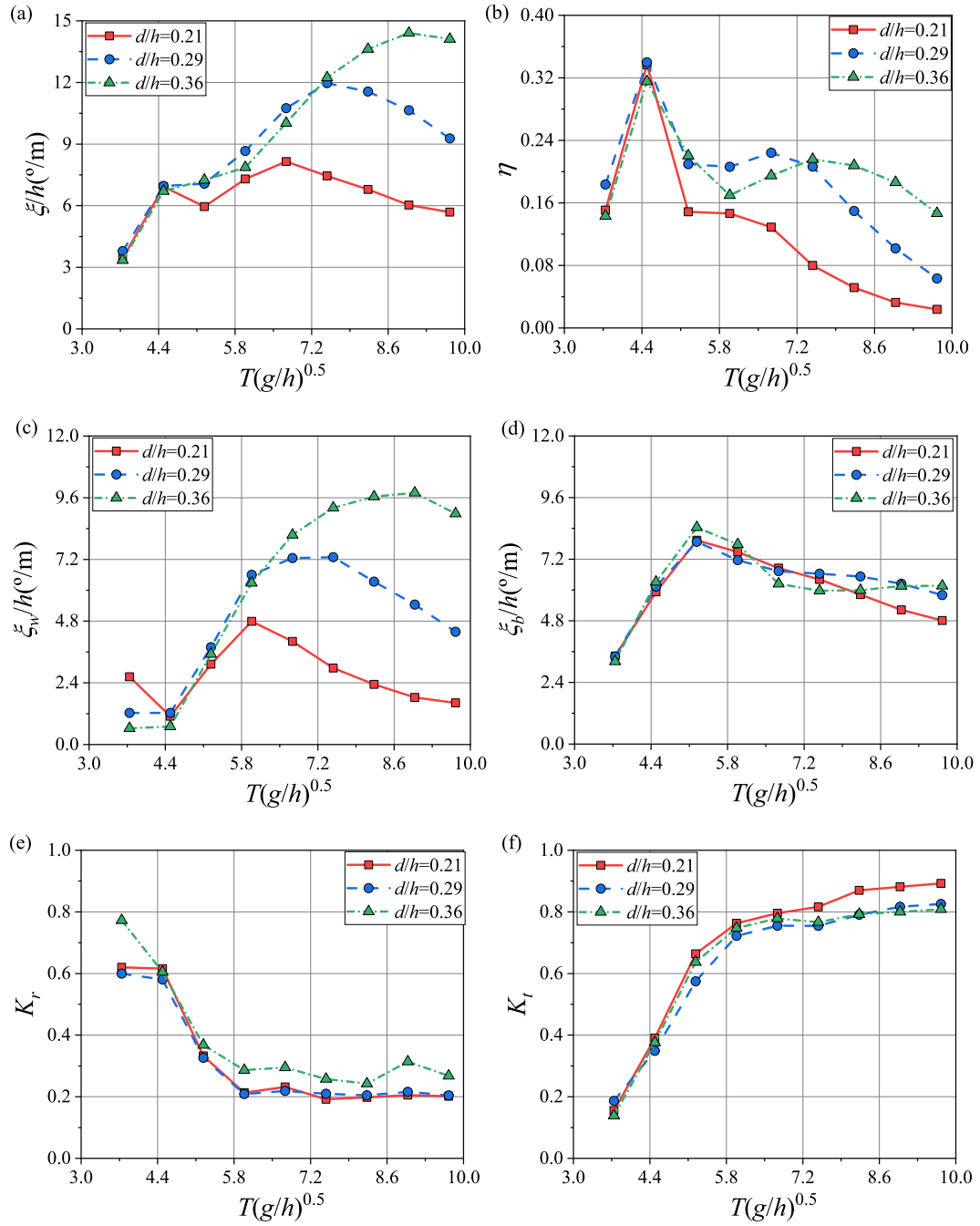
Fig. 10. Variation of (a) relative pitch angle, (b) conversion efficiency, (c) rotated angle of WEC, (d) rotated angle of breakwater, (e) reflection coefficient and (f) transmission coefficient with wave periods at varying WEC drafts.
