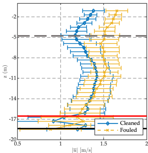
Fig. 15 Ensemble-averaged profiles of along-channel velocity for “cleaned” and “fouled” conditions during ebb tide at 2 m/s inflow conditions, five effective diameters downstream of the turbine. Error bars denote cross-wake variability (1 standard deviation). Grey dashed line denotes turbine hub-depth. Horizontal black line is the bottom. The horizontal red line indicates the depth at which side-lobe contamination from the bottom return begins to contaminate the velocities.
