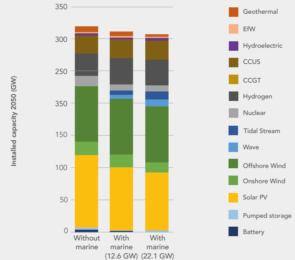
Figure 9 – Installed capacity comparison between scenarios with and without marine energy
