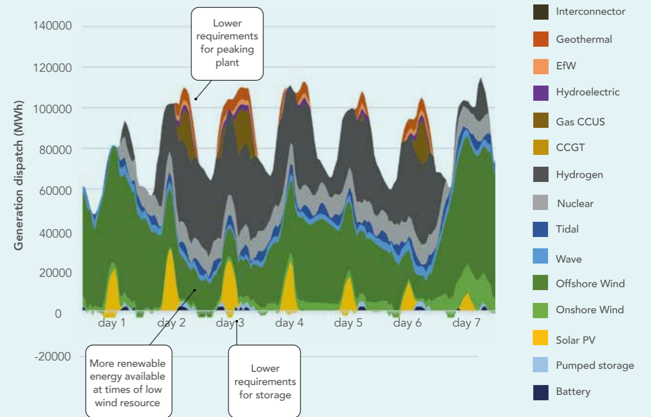
Figure 6b – weekly dispatch from EVOLVE GB economic dispatch model, showing first week in January from 2050 scenarios, with marine energy.
