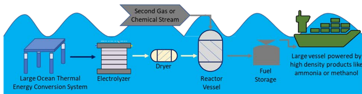
Figure 25. Conceptual framework for powering large oceangoing vessels with high-density products (like ammonia or methanol) derived from H 2 produced from OTEC systems
