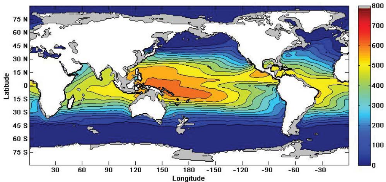
Figure 12. A map of global OTEC resource is plotted in units of kW/(m 3 /s) of cold water pumped from 1-km depth and with assumed system efficiencies.
