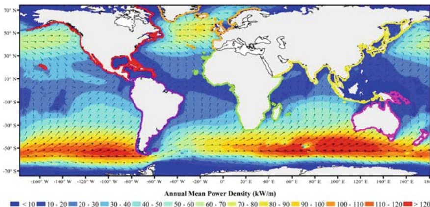
Figure 4. Global resource map of wave power density
