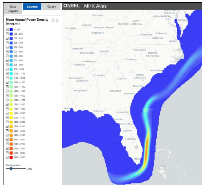
Figure 9. Image of Gulf Stream resource.
