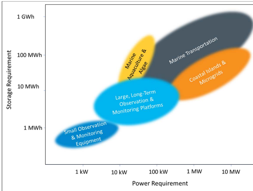
Figure 22. Range of power and storage requirements of the various blue economy applications potentially viable for marine energy-H 2 implementation.
