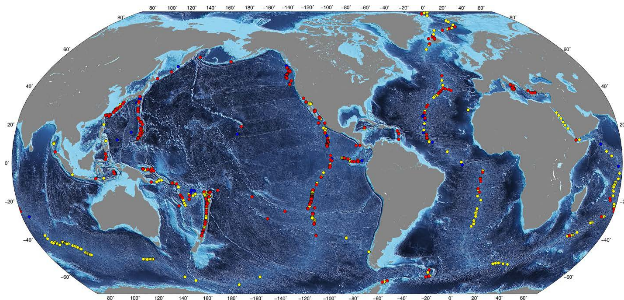
Figure 13. A map of the known, active hydrothermal vent fields from the InterRidge Global Database of Active Submarine Hydrothermal Vent Fields. Colors indicate the reported status of the vent field (red = confirmed active, yellow = inferred active, blue = inactive).
