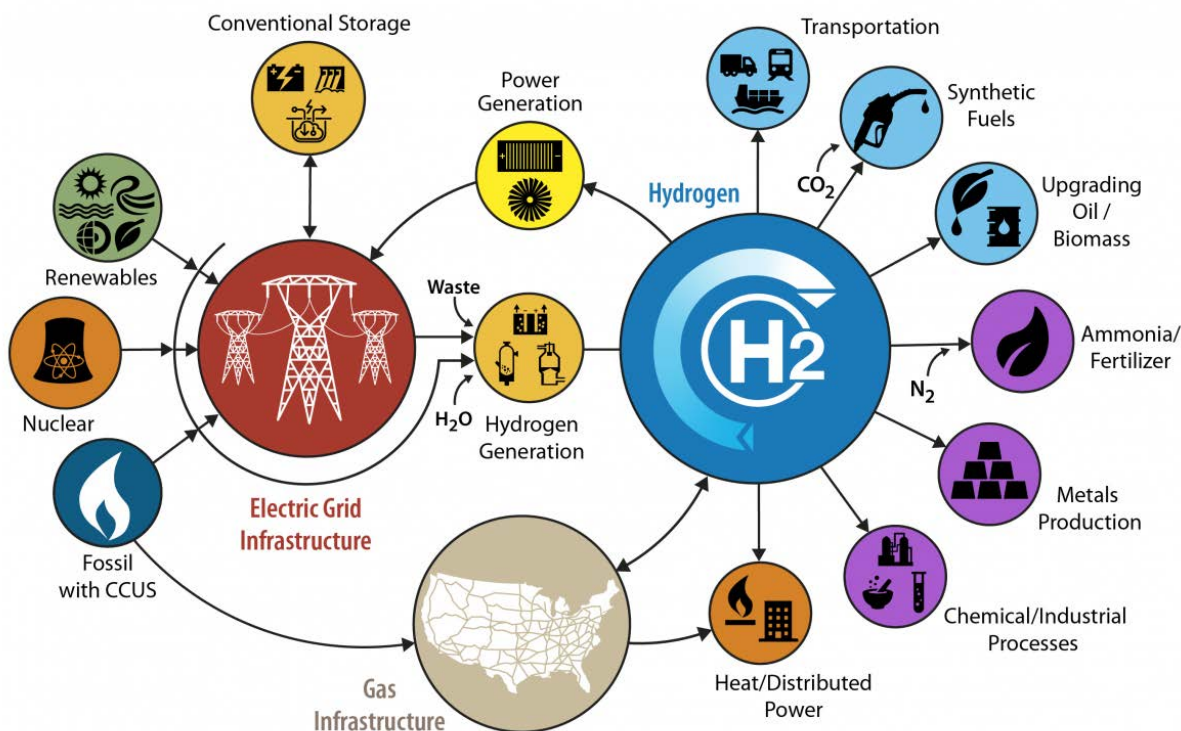
Figure 14. H2@Scale diagram showing hydrogen integration opportunities.
