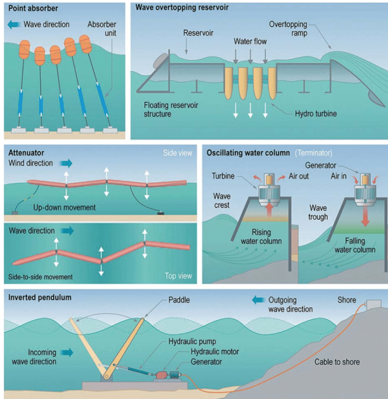
Figure 7. The basic mechanism of common WEC technology types are conceptually illustrated
