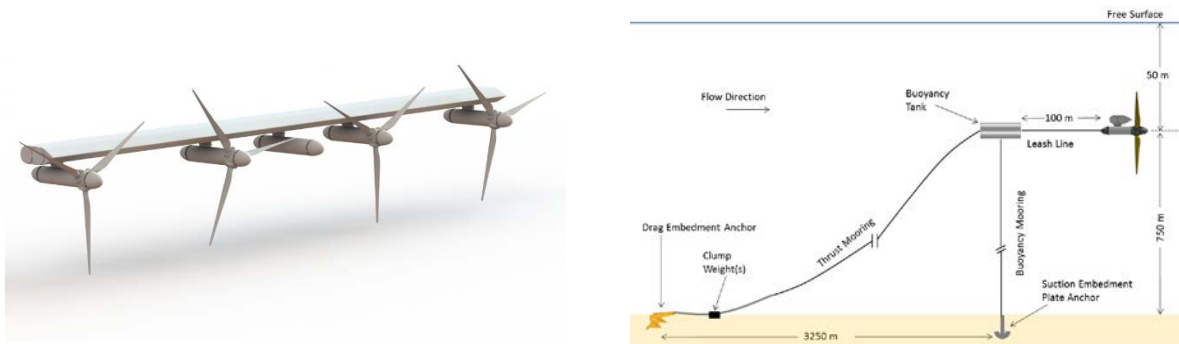
Figure 11. Overall diagram of RM4 (left) and deployment diagram (right).
