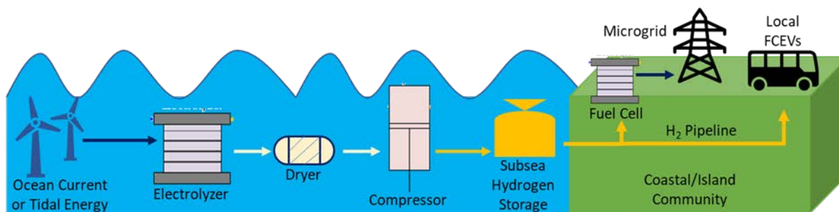
Figure 28. Conceptual framework for powering remote coastal/island communities using local marine energy resources coupled with H 2 systems
