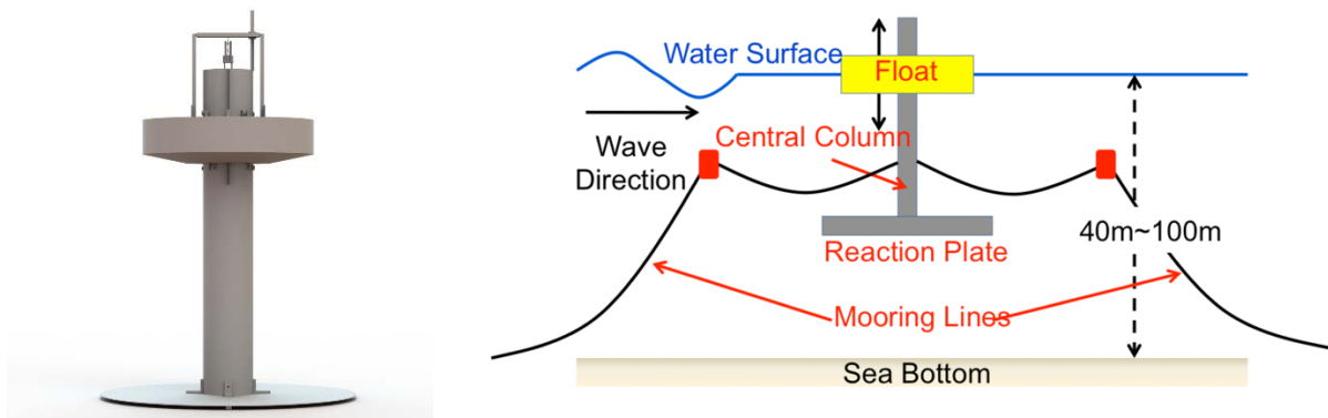
Figure 8. Overall geometry of RM3 (left) and operation diagram (right).
