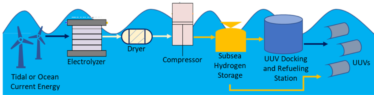
Figure 26. Conceptual framework for powering UUVs using tidal/ocean current energy and H 2 systems. Battery-operated UUVs can be recharged by a central docking and refueling station, while fuel-cell-operated UUVs can be directly fueled by subsea H 2 storage.
