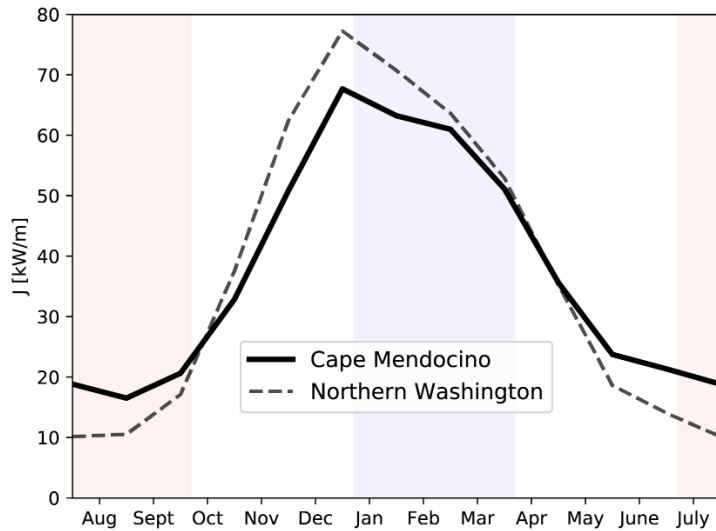
Figure 6. Seasonal variability of wave energy
