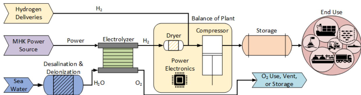
Figure 29. Major subsystems of a marine energy-H 2 project including end uses
