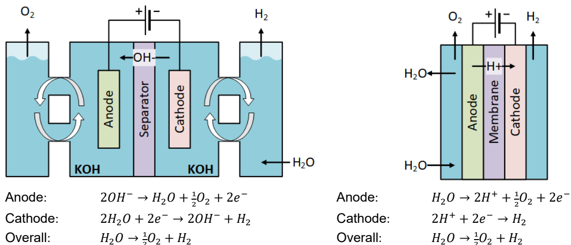
Figure 15. Example diagrams of liquid alkaline (left) and PEM (right) electrolysis cells with the fundamental chemical equations included below each technology.
