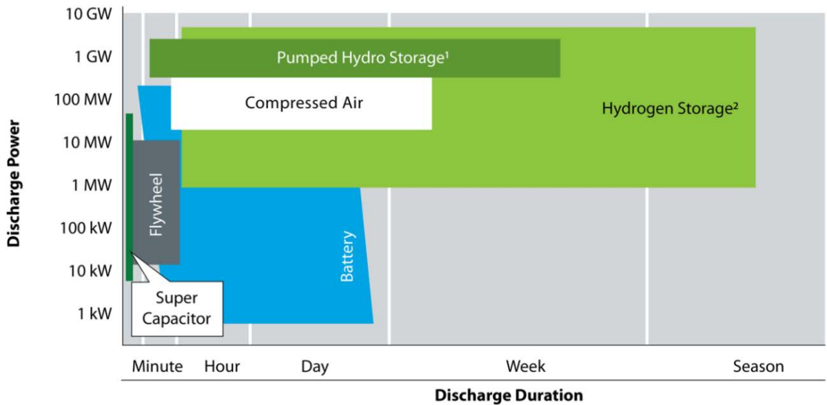
Figure 20. The optimal discharge power and duration characteristics are plotted qualitatively for several prominent energy storage technologies.
