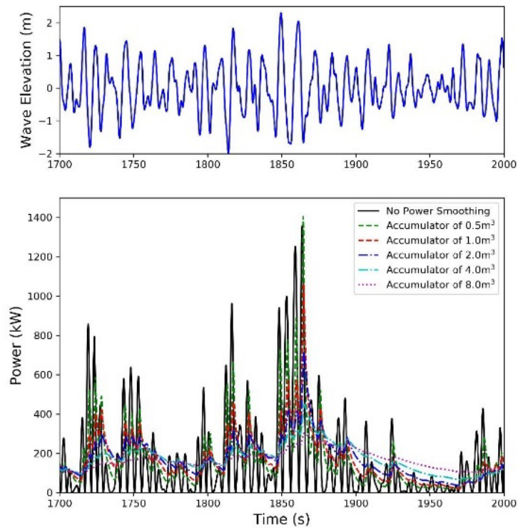
Figure 5. True wave elevation and power timeseries with smoothing effects.
