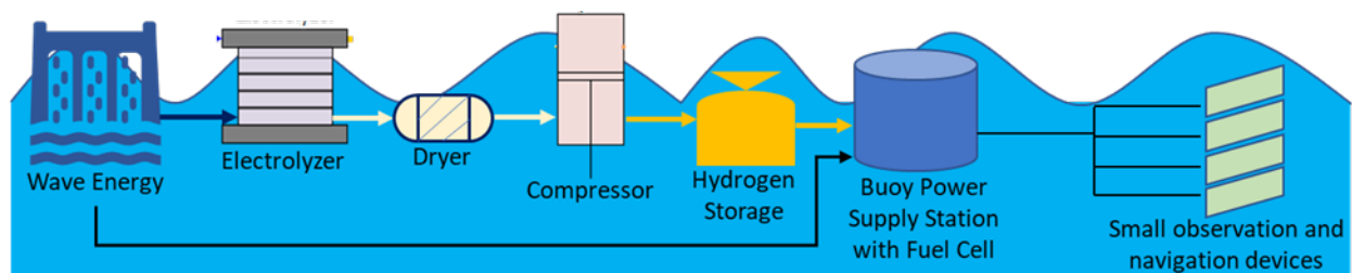
Figure 23. Conceptual framework for powering small coastal observation and navigation devices using wave energy and H 2 systems
