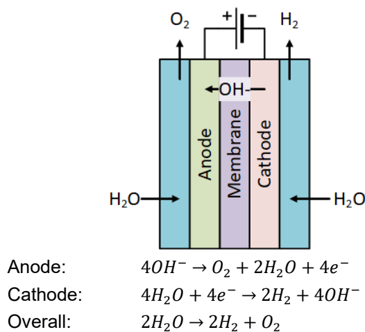
Figure 17. Example of an AEM electrolyzer.
