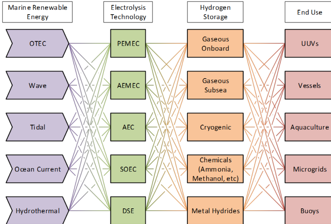
Figure 1. The many possible combinations for a comprehensive marine energy-H 2 system are graphically illustrated for a subset of the possible component technologies.
