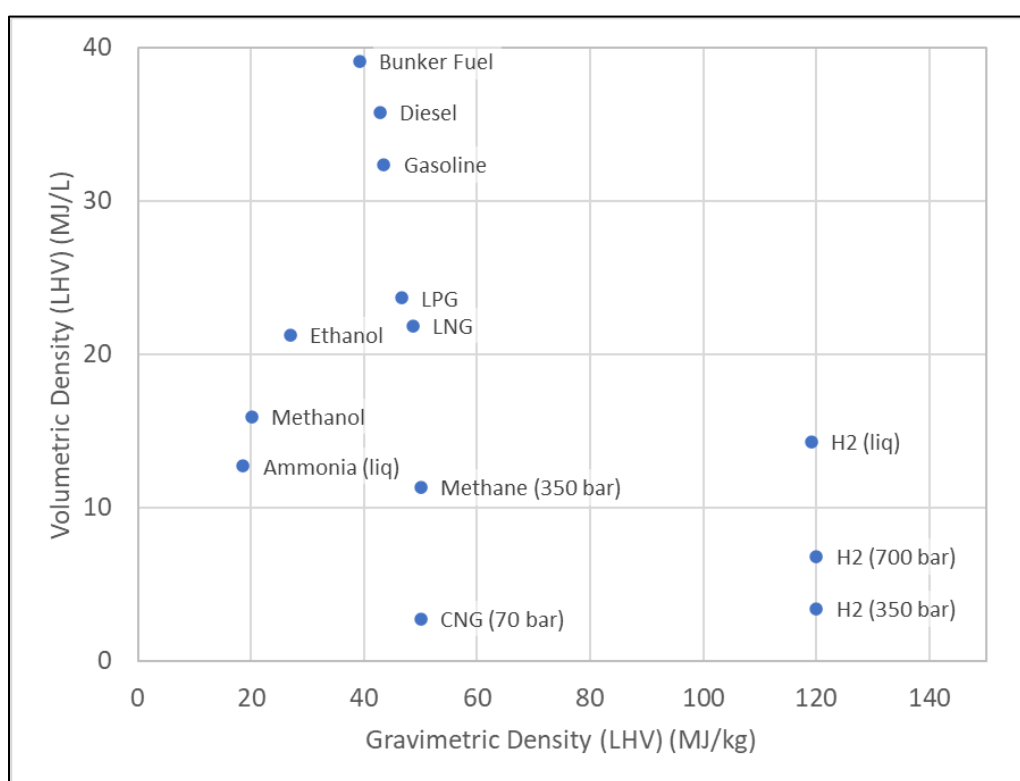
Figure 21. Comparison of gravimetric density and volumetric density for several fuels based on lower heating values.
