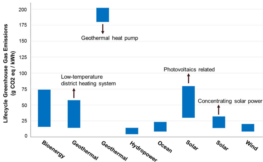
Fig. 12. Estimates of lifecycle GHG emissions of renewable energy technologies (Graphed with the data from [138]).
