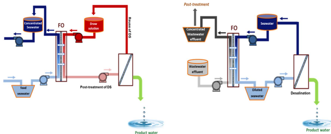
Fig. 7. Layout of two FO processes for seawater desalination: (left: direct FO desalination; right: indirect FO desalination).
