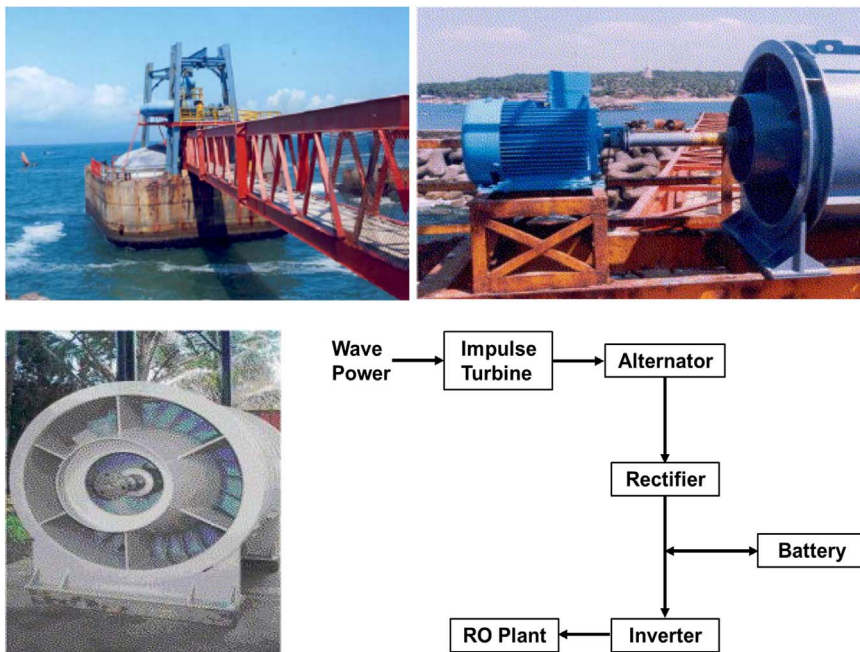
Fig. 6. OWC system for seawater desalination at Vizhinjam in India (upper left: the panoramic view; upper right: permanent magnet brush less alternator; lower left: Impulse turbine; lower right: the flow-chat of OWC system) [87].
