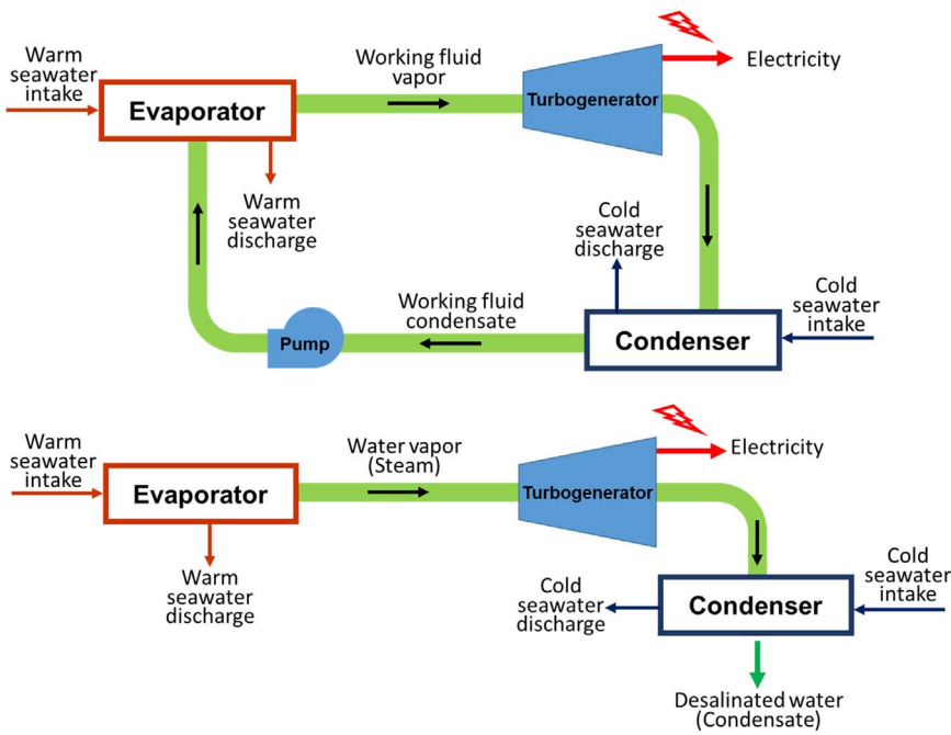
Fig. 5. Schematic diagram of OTEC and integrated seawater desalination processes (upper, close-cycle; lower, open-cycle using seawater).
