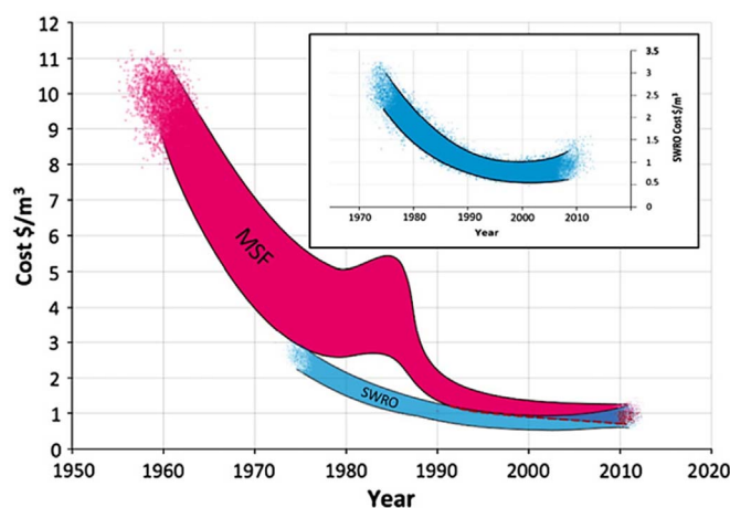
Fig. 3. Trends in the cost of seawater desalination [15].
