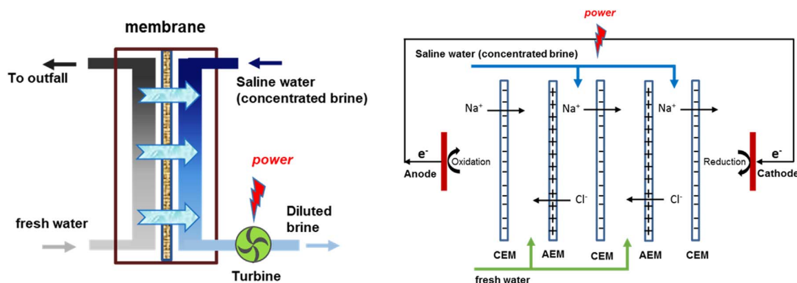
Fig. 8. The flow chat of PRO (left) and RED (right; CEM: cation exchange membrane; AEM: anion exchange membrane).
