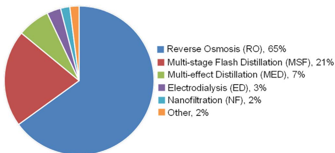
Fig. 1. Total worldwide installed desalination capacity by technology [1].
