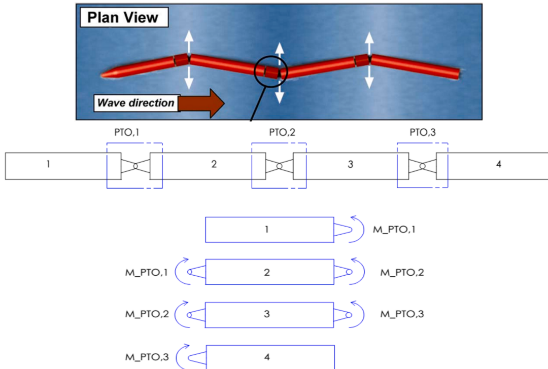
Fig. 1. Pelamis energy converter schematic and the free vibration diagram of its different components; Plan view (upper panel); Free vibration diagram of Pelamis components (bottom panel) [37].
