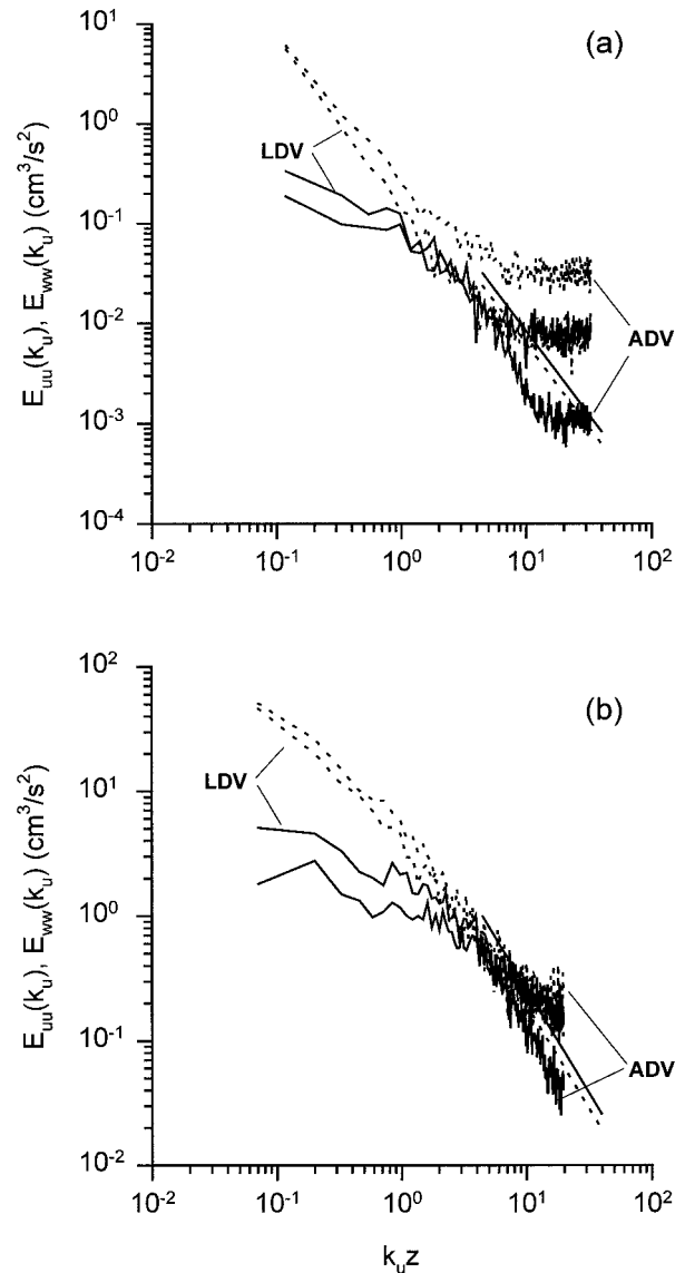
FIG. 7. Both ADV and LDV turbulence velocity spectra along the horizontal [ E_{uu}(k_u) , solid lines] and vertical [ E_{ww}(k_w) , dotted lines] for two typical runs with boundary Reynolds numbers ( u_* \kappa z / \nu ) 56 and 528 for diagrams (a) and (b), respectively. Flow conditions for the spectra shown. Panel (a): h = 25.5 cm; z = 3.1 cm, U = 7.4 cm s -1 , and u_* = 0.45 cm s -1 . Panel (b): h = 25.0 cm, z = 8.1 cm, U = 32.1 cm s -1 , and u_* = 1.63 cm s -1 . Shear velocities u_* were derived using Eq. (21) with Reynolds stress \langle u'w' \rangle values based on the ADV-recorded velocities. [Note: Straight lines represent Kolmogorov's turbulence spectra model, Eq. (27), for k_u z > 4.5 .]
