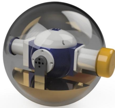
Figure 1 - Small WITT in Sealed Housing
