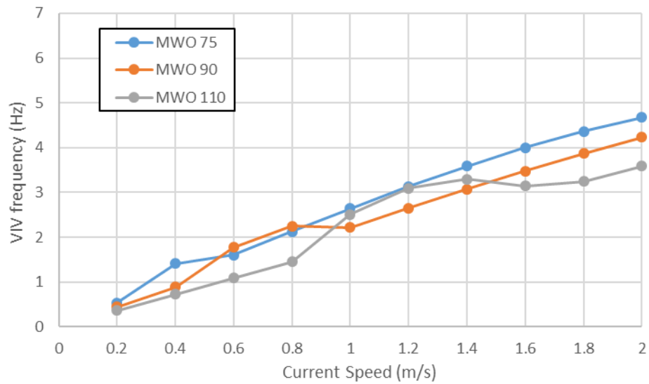
Figure 11 – WITT VIV Frequency for 3 pipe diameters (75mm 90mm 110mm) using the Milan Wake Oscillator [MWO]
