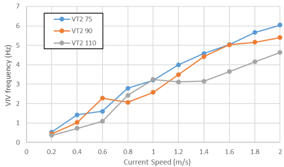
Figure 17 – WITT VIV Frequency for 3 pipe diameters (75mm 90mm 110mm) using Vortex Tracking 2 [VT2]
