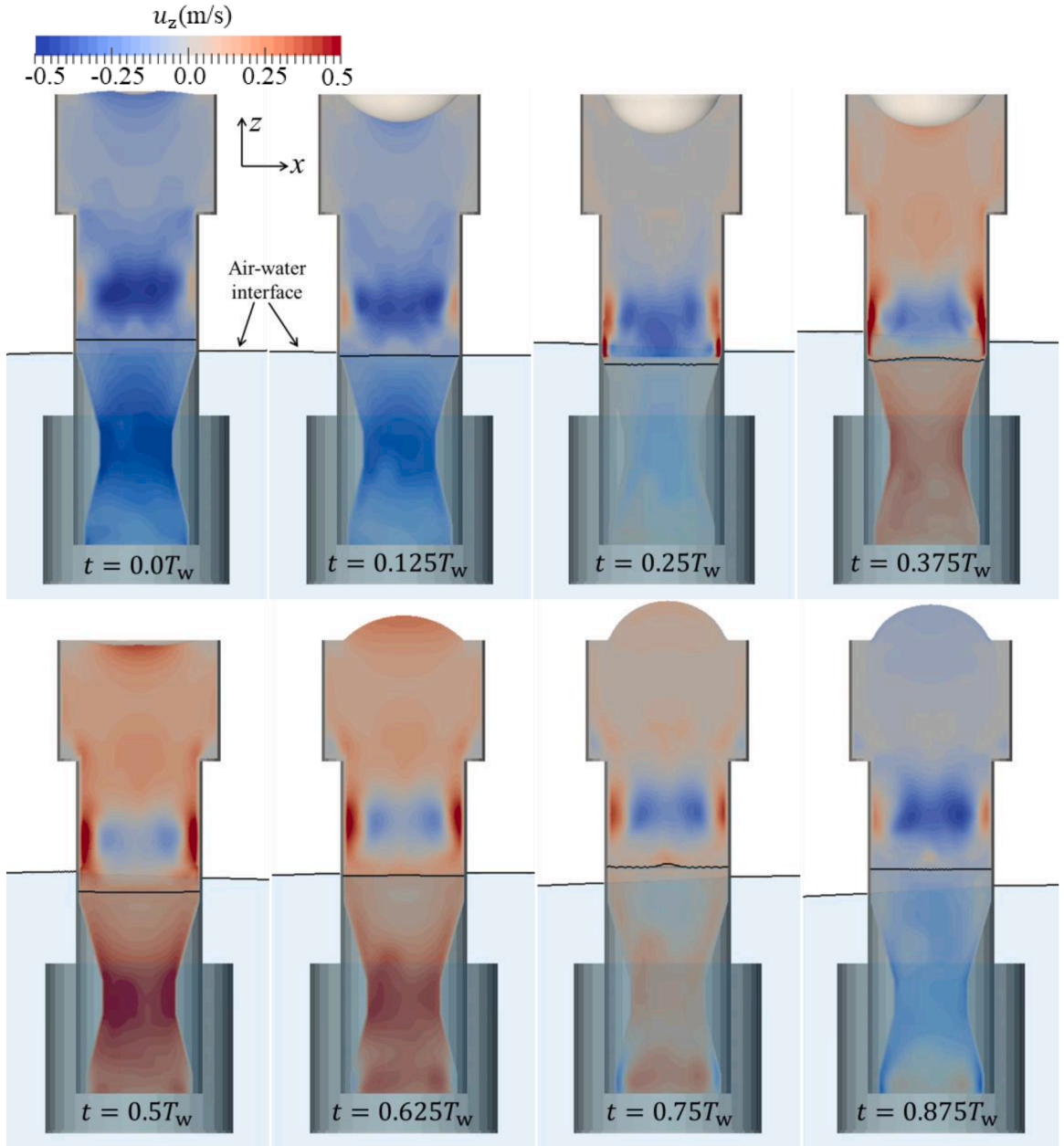
Fig. 12. Velocity field in the x - z plane at selected time instants over one wave period in load case LC2 at resonant frequency f_w = 0.4 Hz.
