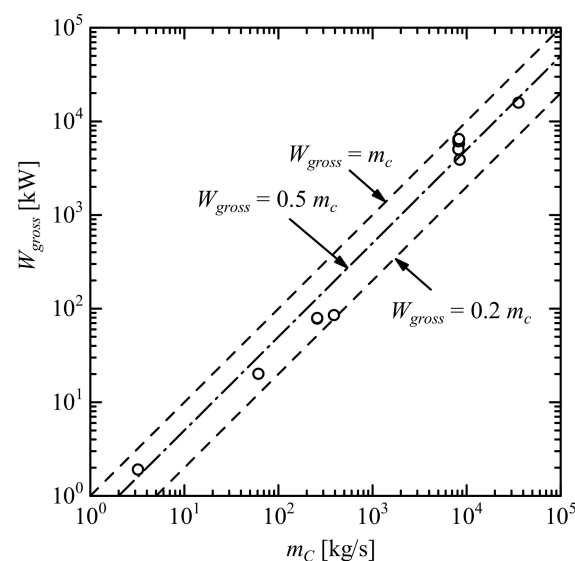
Figure 6. Relation between deep seawater flow rate and gross power in design. The gross power is roughly proportional to the mass flow rate of deep seawater.
