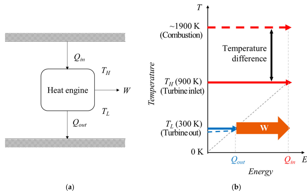
Figure 1. Concept of a heat engine driven by heat and the relationship between temperature and energy in conventional thermal power plants; (a) concept of a heat engine; (b) conceptual T – E diagram. The heat source is the combustion of the fuel. The work of the heat engine is the difference between Q_{in} and Q_{out} .
