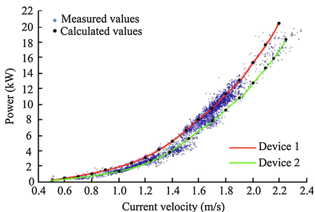
Fig. 2 Curves of output power of Device 1 and Device 2
