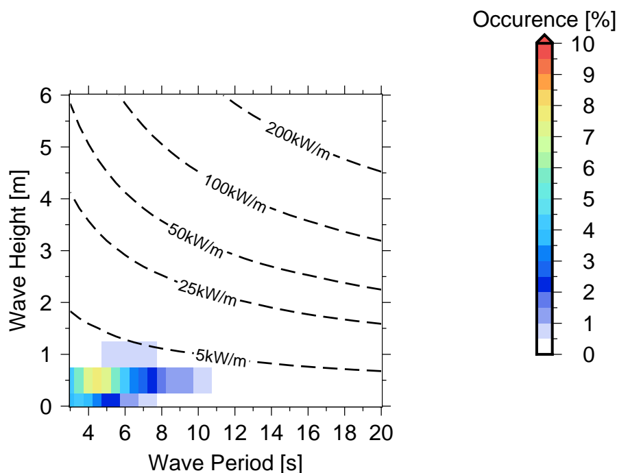
Figure 10 Occurrences of sea states in Avarua passage .
