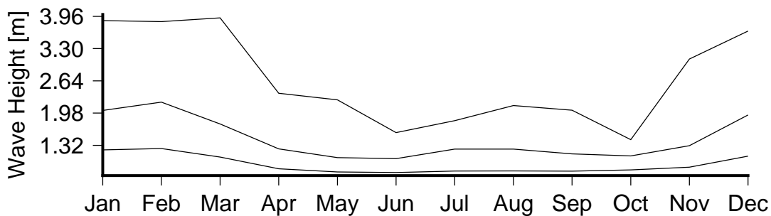
Figure 7 Monthly variation in large waves (90th percentile)(lower curve), severe waves (99th percentile) (middle curve) and the largest wave(upper curve) in Avarua passage.
