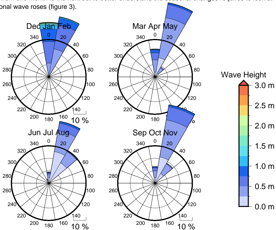
Figure 3 Seasonal wave roses for Avarua passage
