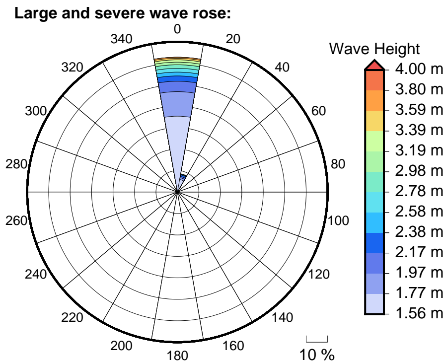
Figure 6 Large, severe and extreme wave roses for Avarua passage
