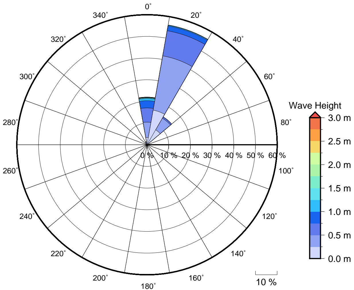
Figure 2 Annual wave rose for Avarua passage. Note that direction are where the wave are coming from .
