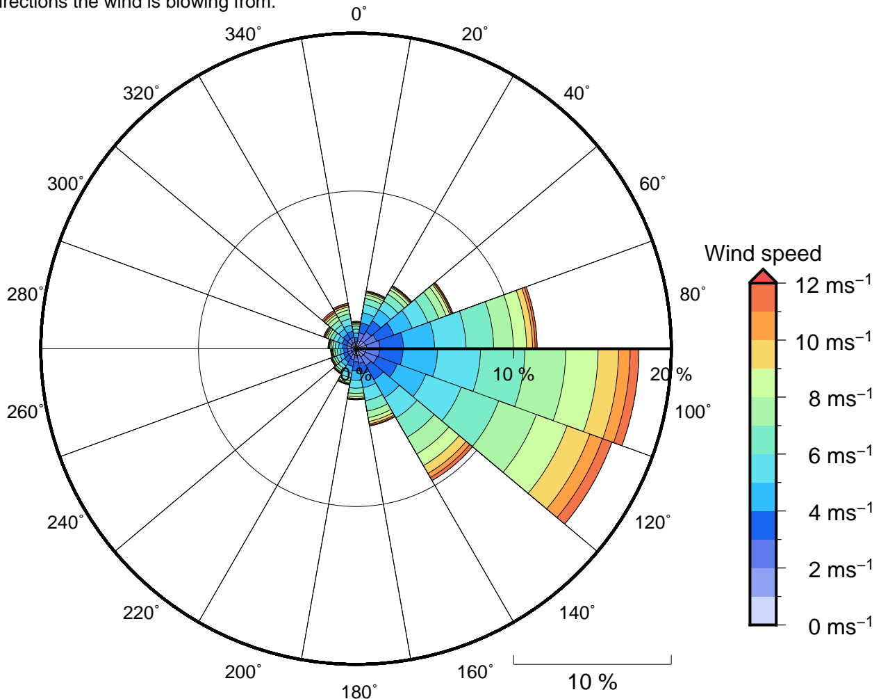
Figure 11 Annual wind rose for Avarua passage. Note that directions are where the wind is coming from.
