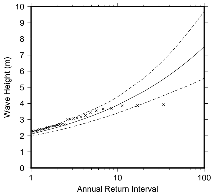
Figure 9 Extreme wave distribution for Avarua passage. The crosses represents the wave events that occurred since 1979. The plain line is the statistical distribution that best fit the past wave events. The dotted line show the upper and lower high confidence of the fit, there is a 95% chance that the fitted distribution lie between the two dashed lines.
