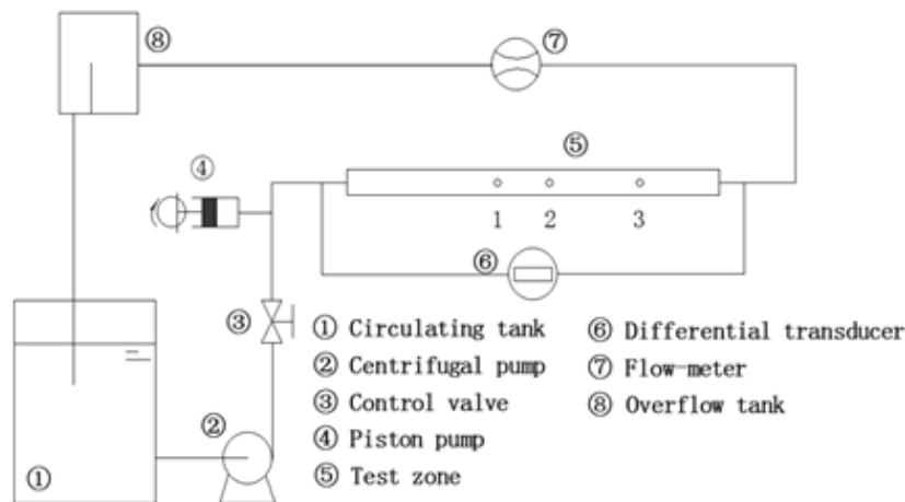
Fig. 1 Schematic diagram of the experimental system
