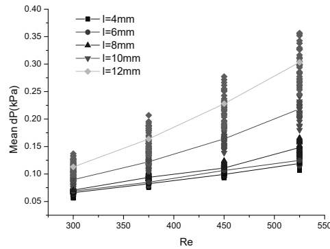
Fig. 5 Mean pressure drop for the whole flow regime
