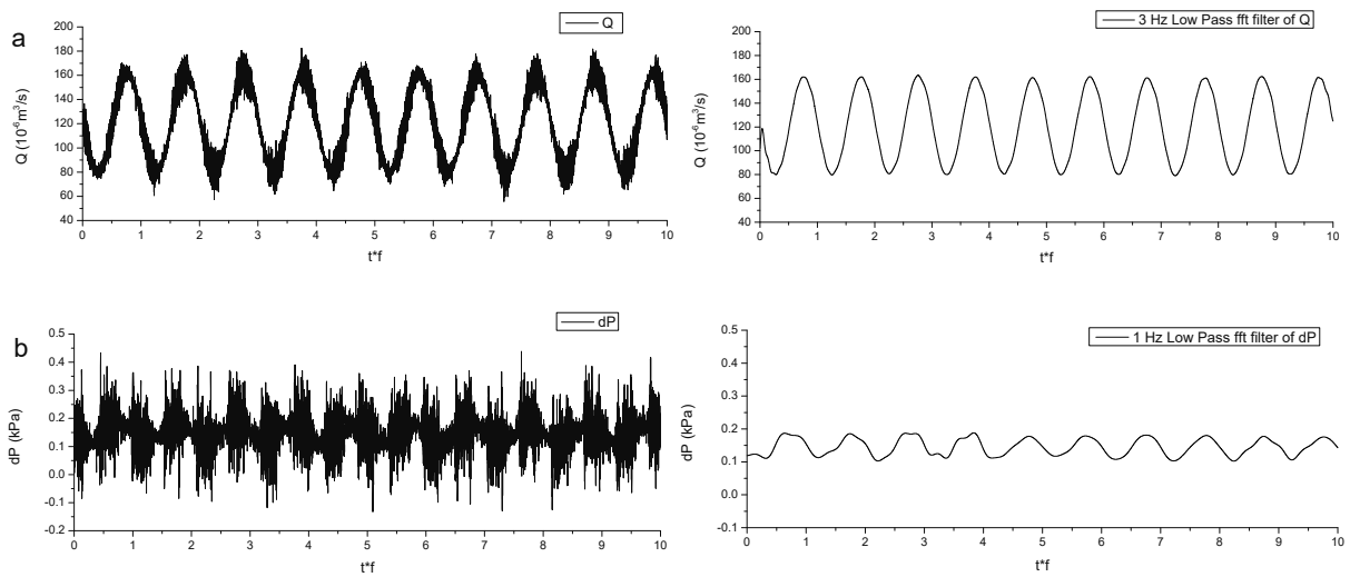
Fig. 4 Sampling data filter for Q and pressure drop
