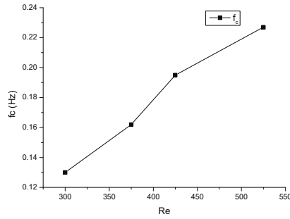
Fig. 7 Critical frequency of pulsatile flow in different Reynold number
