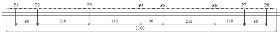
Fig. 2 The measuring point positions on the grooved plate
