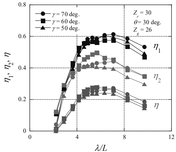
Fig. 5 Changes in efficiencies at time-averaged rotational speed N_t = 700 rpm.
