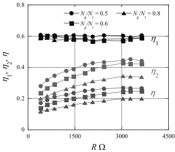
Fig. 6 Change in efficiencies due to electric resistor.
