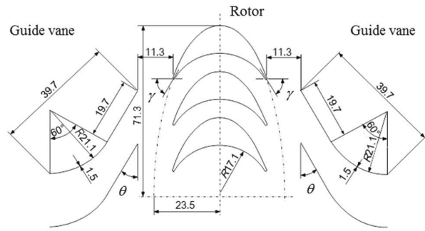
Unit : mm Fig. 3 Configuration of rotor and guide vane.
