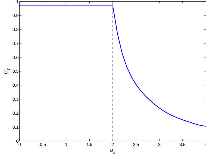
Figure 8.4: Thrust coefficient C_T vs. array flow speed u_a for the turbine in blockage ratio B = 0.2 .
