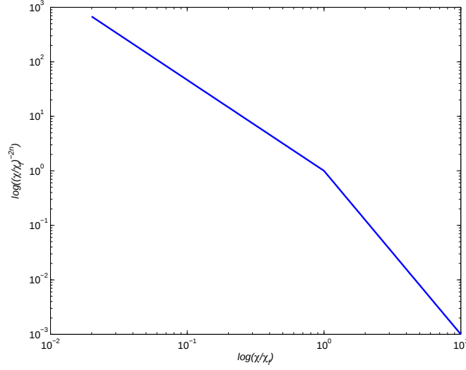
Figure 5.4: Variation of the function \frac{\chi}{\chi_f}^{-2n} as \frac{\chi}{\chi_f} increases which corresponds to eddies becoming smaller.
