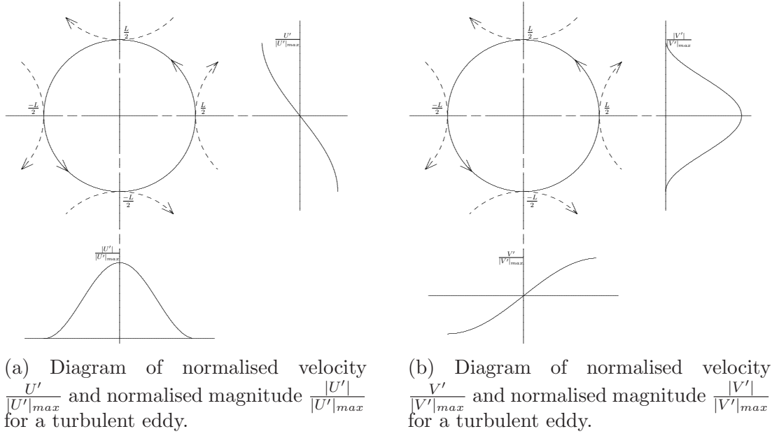
Figure 5.3: Normalised velocity and magnitude components of a turbulent eddy with diameter L . The dashed arrows represent the rotation of neighbouring eddies.
