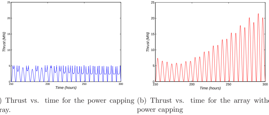
Figure 8.12: Comparison of thrust vs. time curves for the turbine array with (blue) and without (red) power capping implemented in a channel forced by the M2 and S2 tidal constituents.
