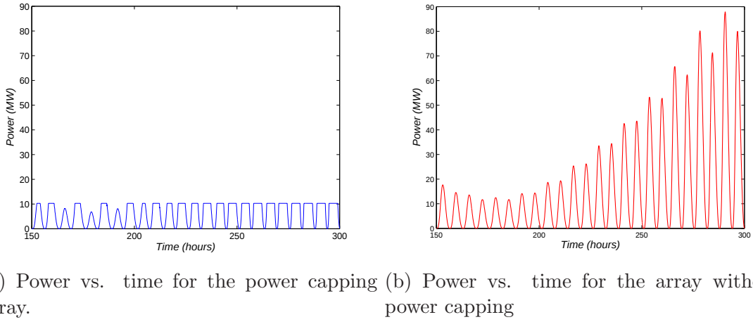
Figure 8.13: Comparison of power vs. time curves for the turbine array with (blue) and without (red) power capping implemented in a channel forced by the M2 and S2 tidal constituents.
